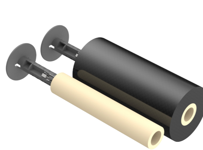
Ribbon Adapter for Notchless Ribbon Cores 205-188-010 12.7 mm (0.5 in) Ribbon Core Adapters
